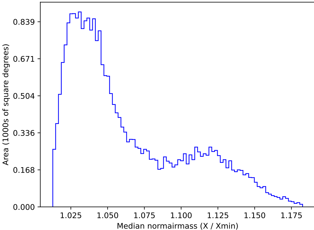
smc_lmc_v3.3_10yrs All sky g band: Median normairmass
