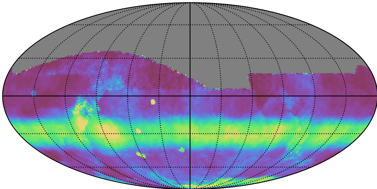
smc_lmc_v3.3_10yrs All sky all bands: Median normairmass
