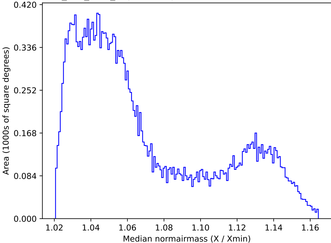
smc_lmc_v3.3_10yrs All sky all bands: Median normairmass
