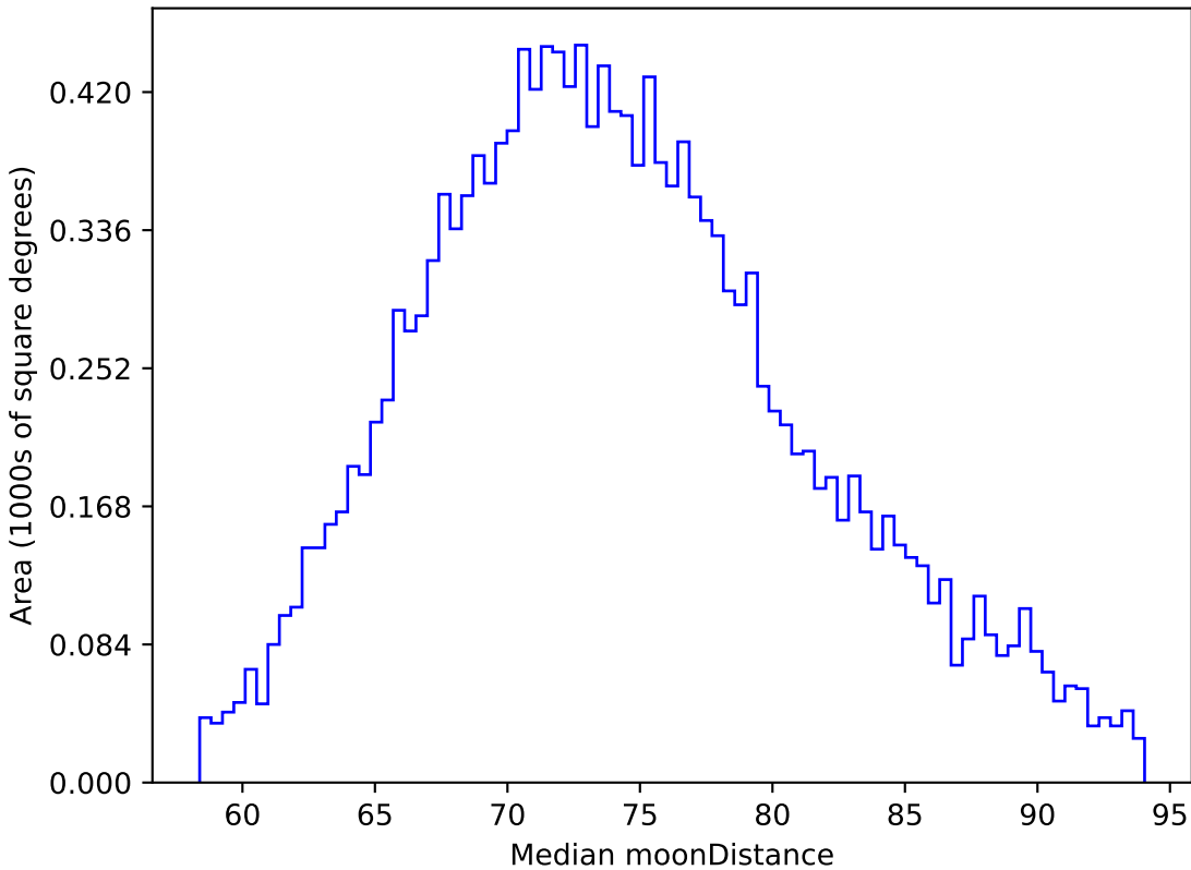
smc_lmc_v3.3_10yrs WFD z band: Median moonDistance
