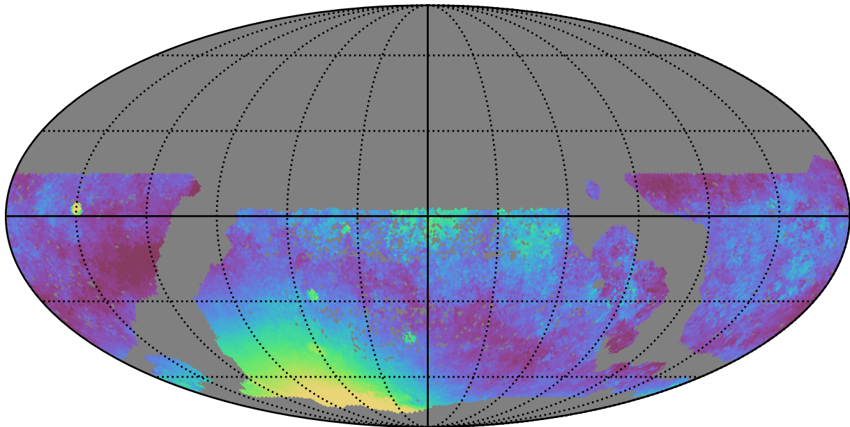
smc_lmc_v3.3_10yrs WFD y band: Median moonDistance
