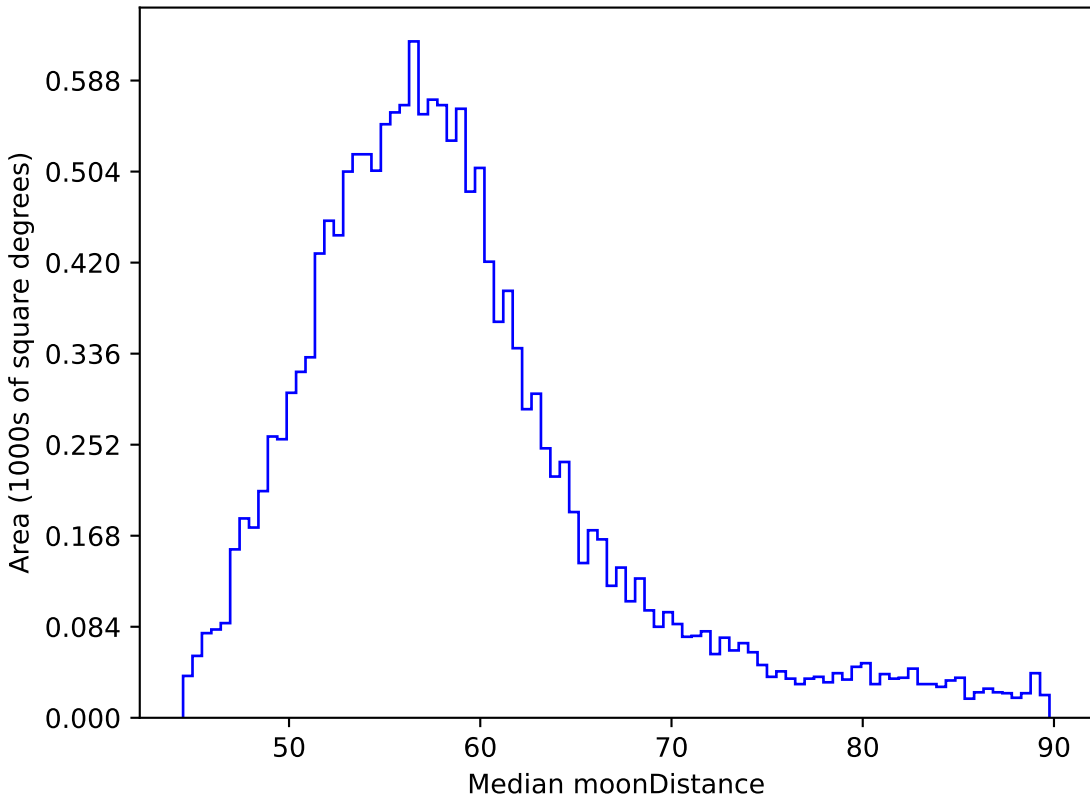
smc_lmc_v3.3_10yrs WFD y band: Median moonDistance
