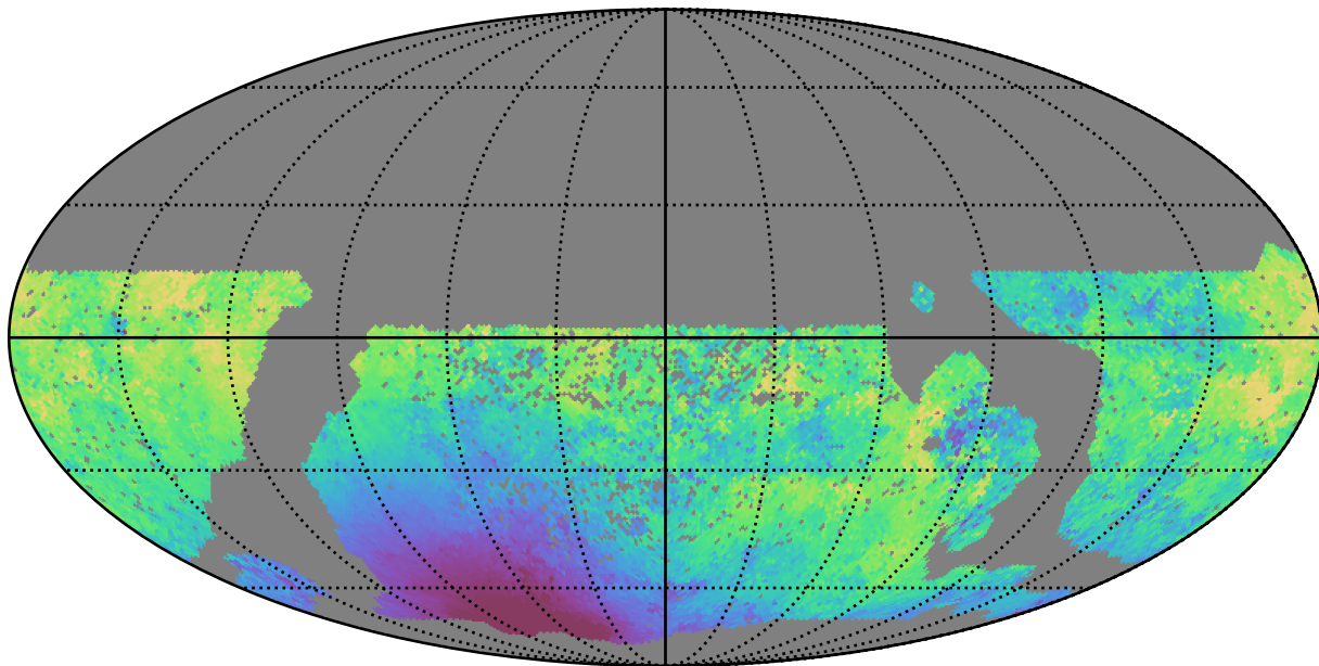
smc_lmc_v3.3_10yrs WFD u band: Median moonDistance
