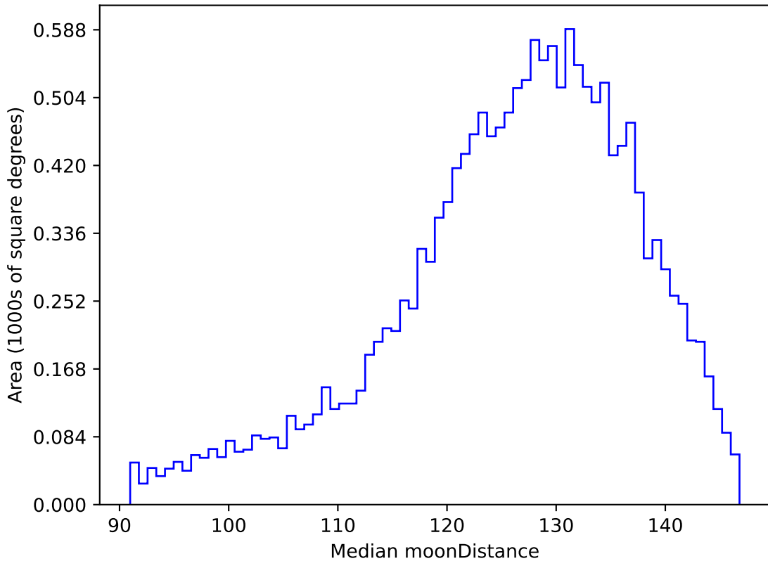
smc_lmc_v3.3_10yrs WFD u band: Median moonDistance
