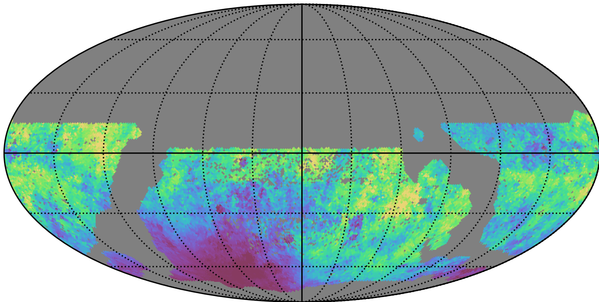
smc_lmc_v3.3_10yrs WFD r band: Median moonDistance
