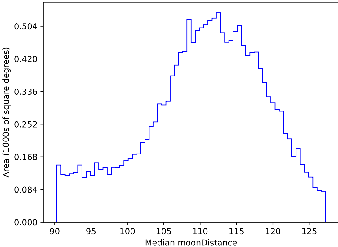
smc_lmc_v3.3_10yrs WFD r band: Median moonDistance
