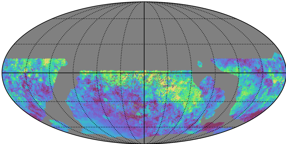
smc_lmc_v3.3_10yrs WFD i band: Median moonDistance
