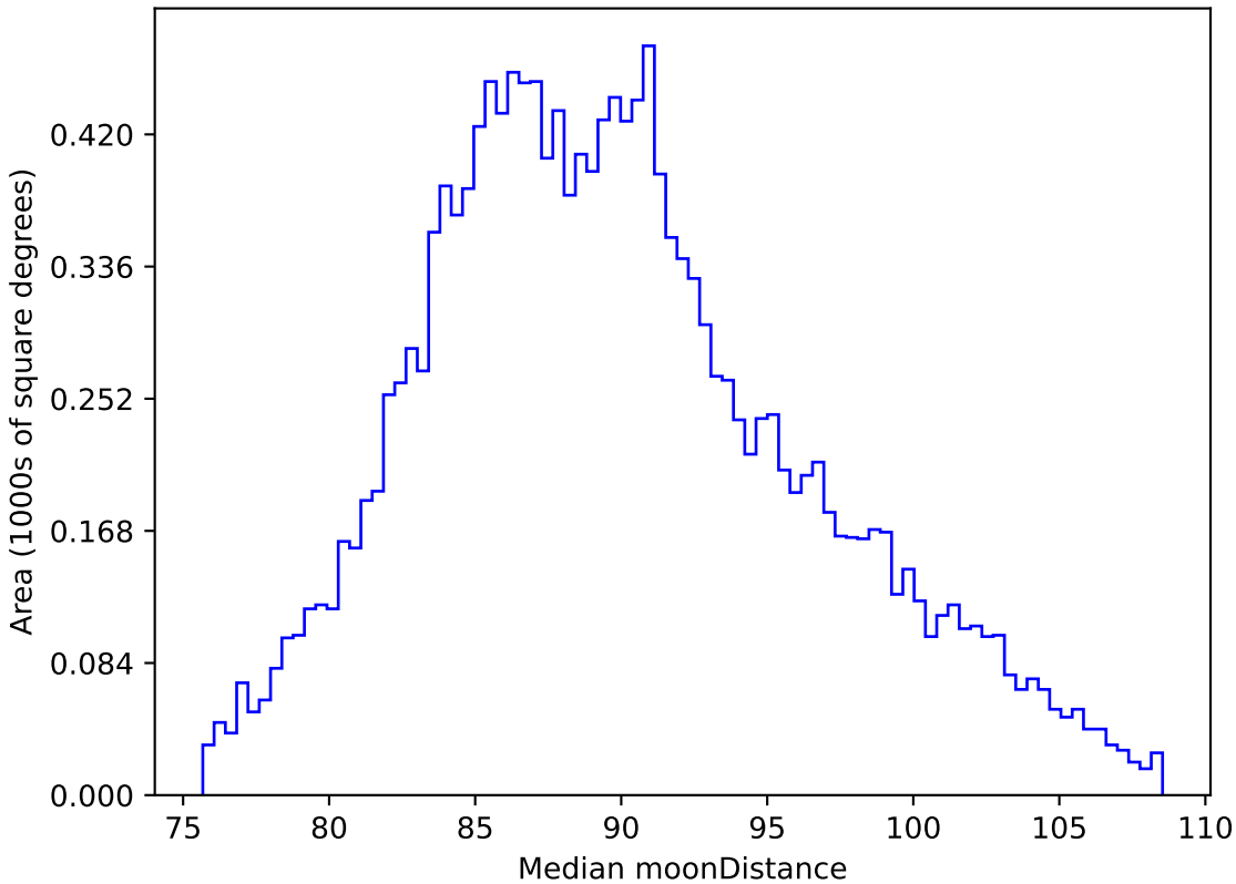
smc_lmc_v3.3_10yrs WFD i band: Median moonDistance
