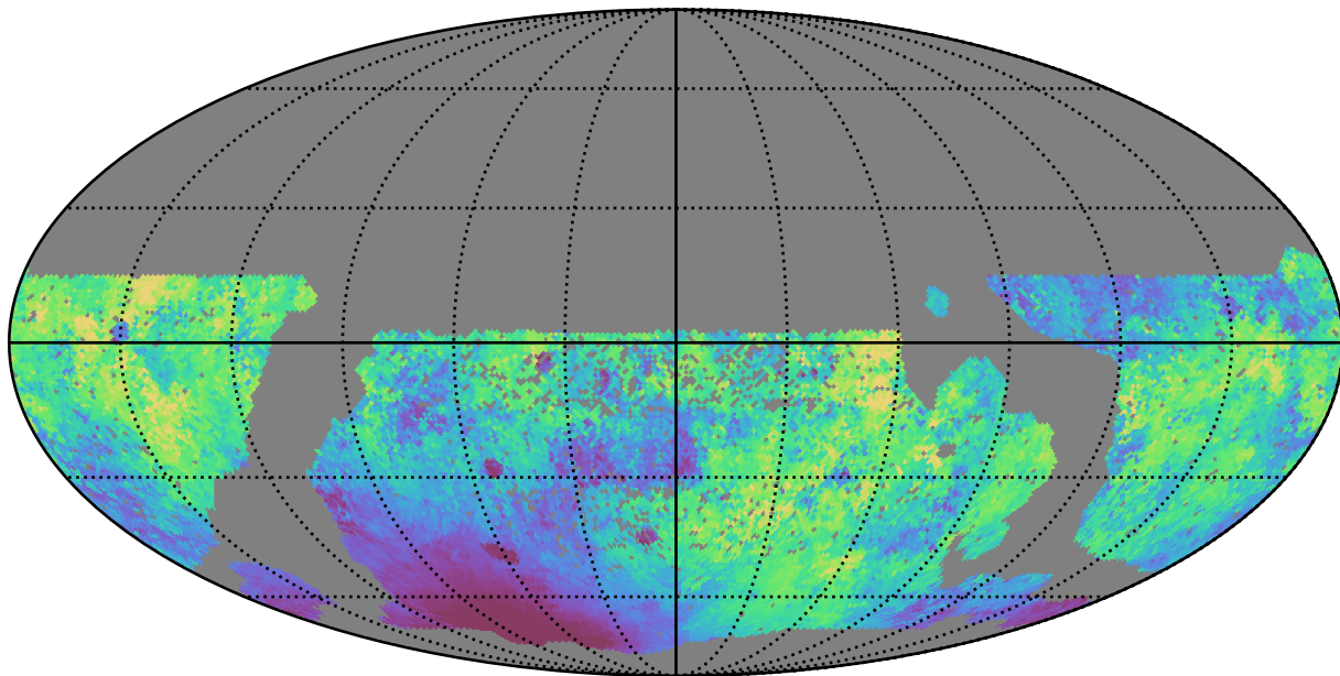
smc_lmc_v3.3_10yrs WFD g band: Median moonDistance
