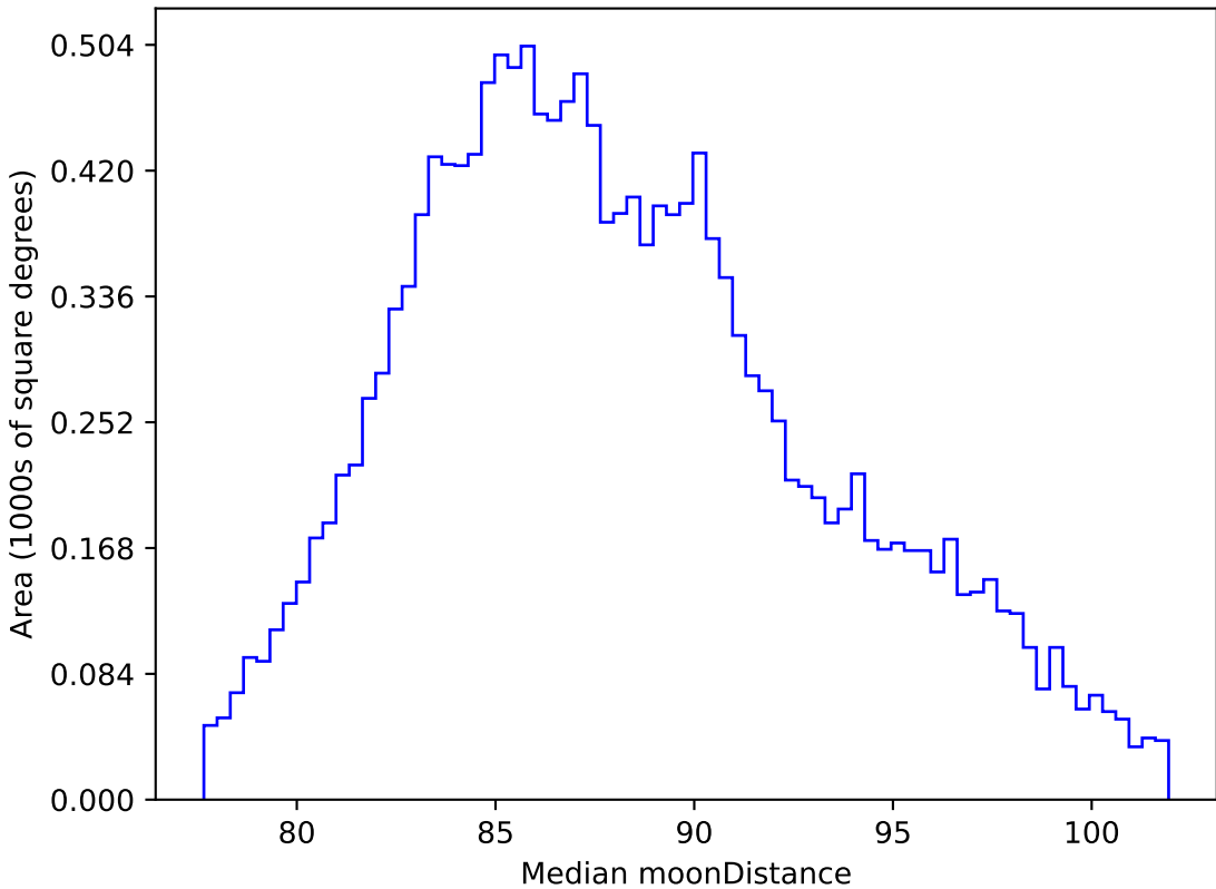
smc_1mc_v3.3_10yrs WFD all bands: Median moonDistance
