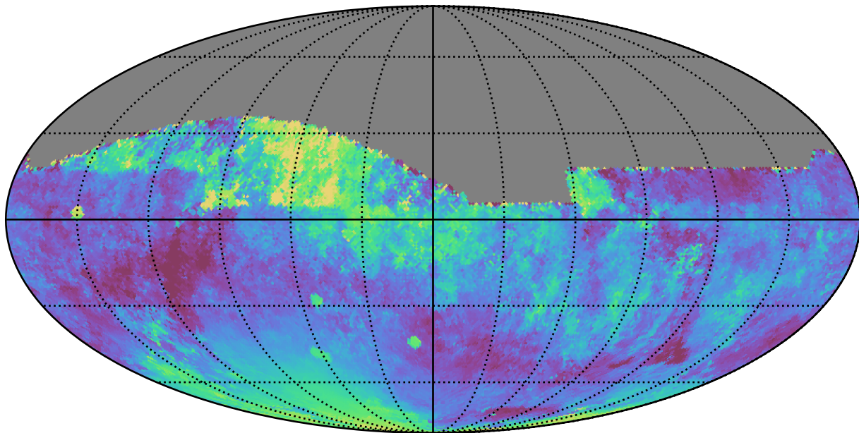
smc_lmc_v3.3_10yrs All sky z band: Median moonDistance
