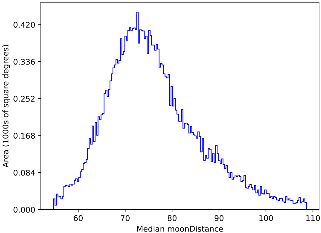
smc_lmc_v3.3_10yrs All sky z band: Median moonDistance
