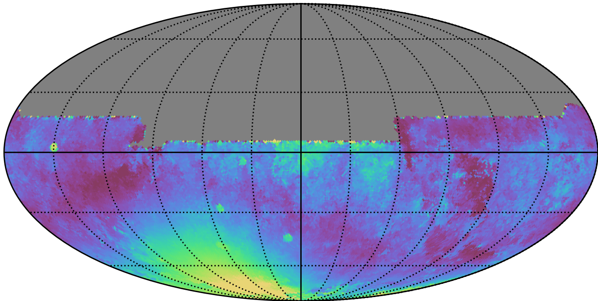
smc_lmc_v3.3_10yrs All sky y band: Median moonDistance
