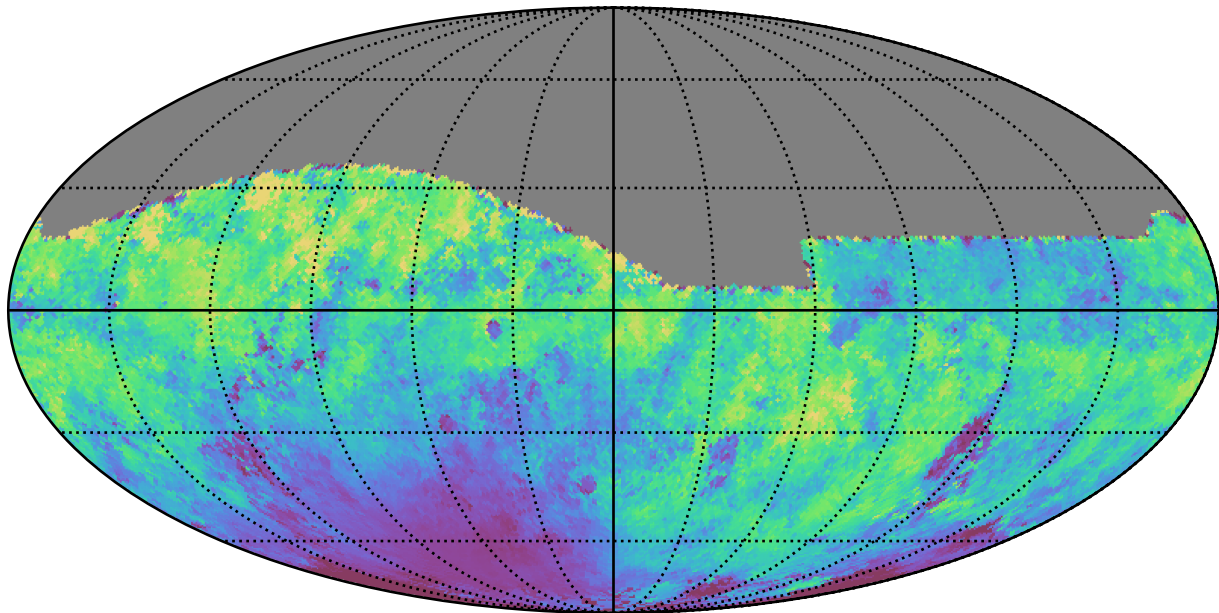
smc_lmc_v3.3_10yrs All sky r band: Median moonDistance
