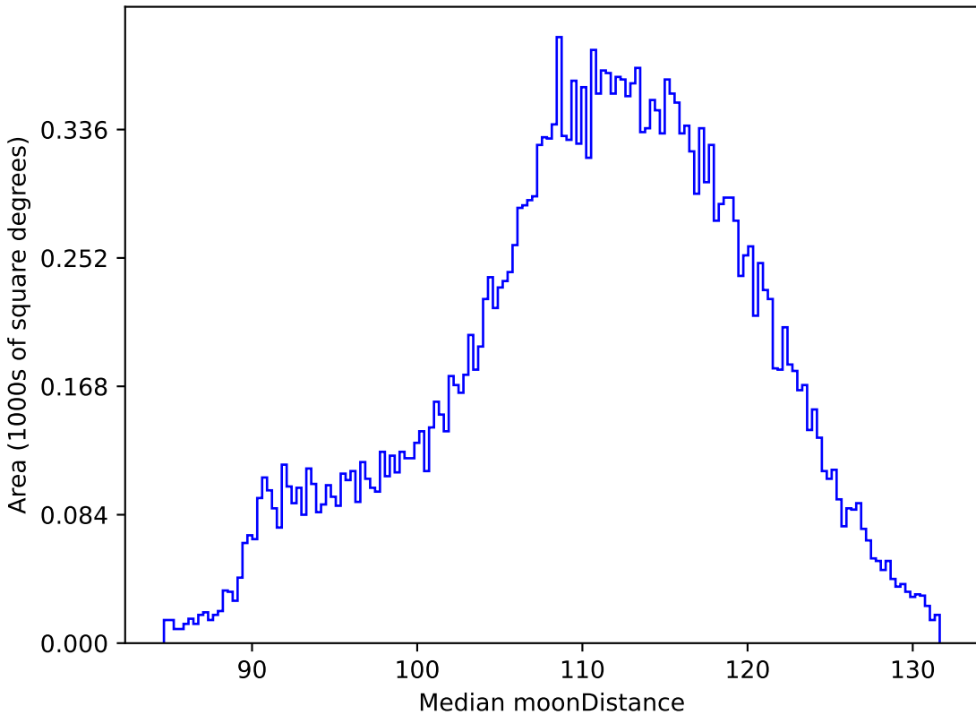
smc_lmc_v3.3_10yrs All sky r band: Median moonDistance
