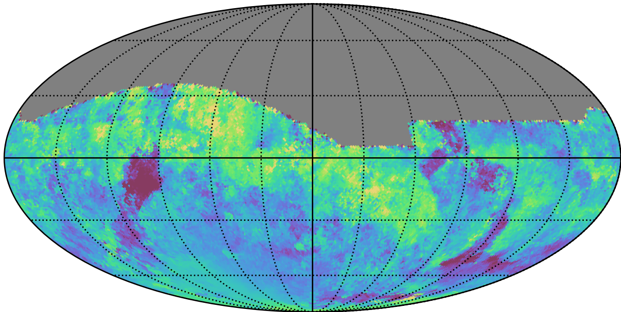
smc_lmc_v3.3_10yrs All sky i band: Median moonDistance
