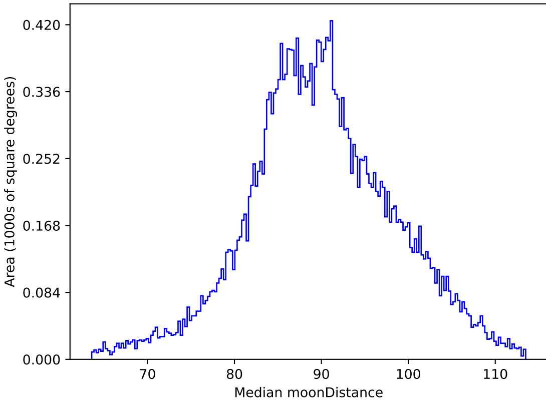
smc_lmc_v3.3_10yrs All sky i band: Median moonDistance
