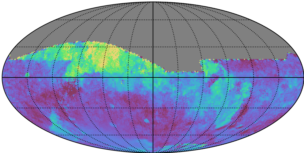
smc_lmc_v3.3_10yrs All sky all bands: Median moonDistance
