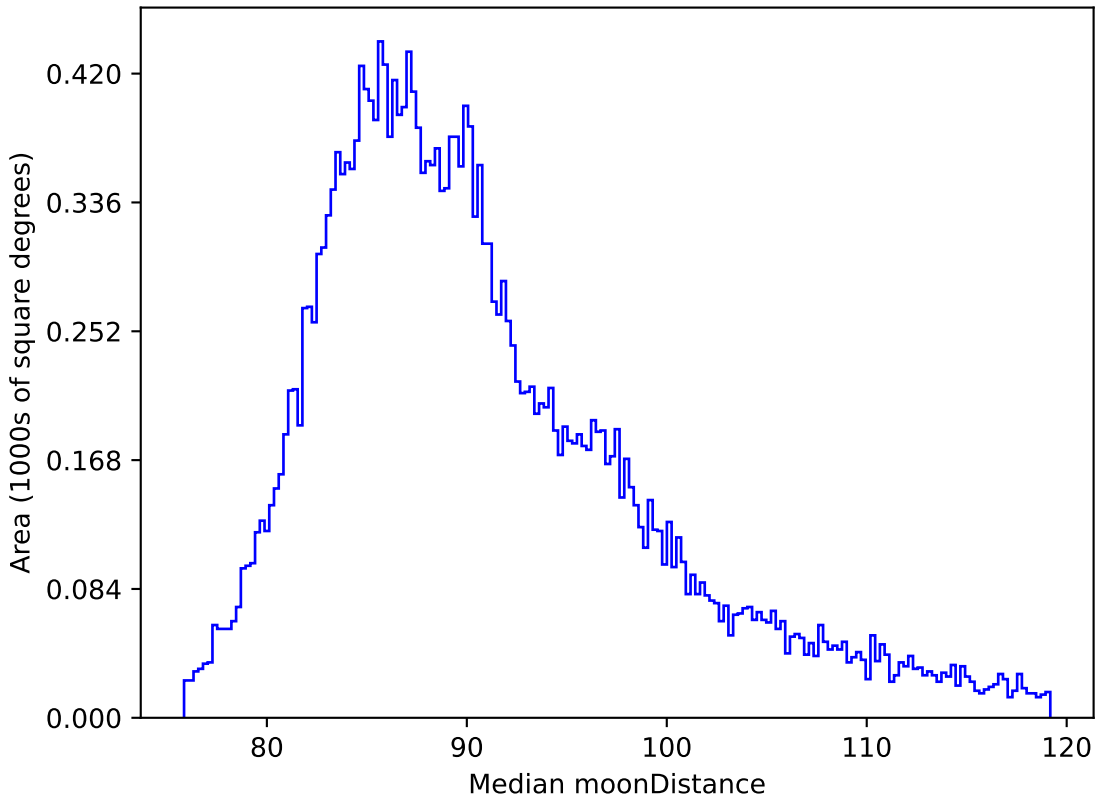
smc_lmc_v3.3_10yrs All sky all bands: Median moonDistance
