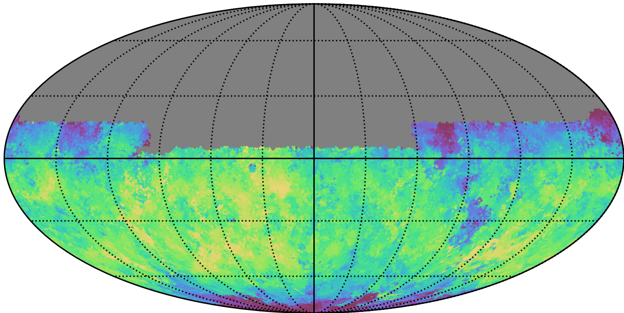
smc_lmc_v3.3_10yrs Yr 1 y band: Median fiveSigmaDepth
