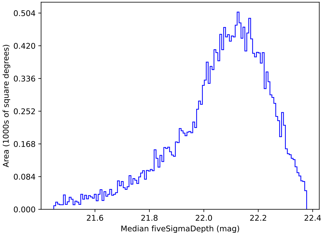
smc_lmc_v3.3_10yrs Yr 1 y band: Median fiveSigmaDepth
