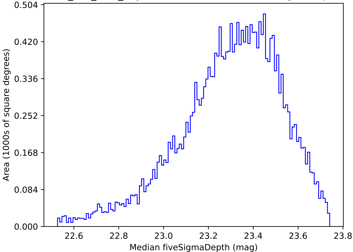
smc_lmc_v3.3_10yrs Yr 1 u band: Median fiveSigmaDepth
