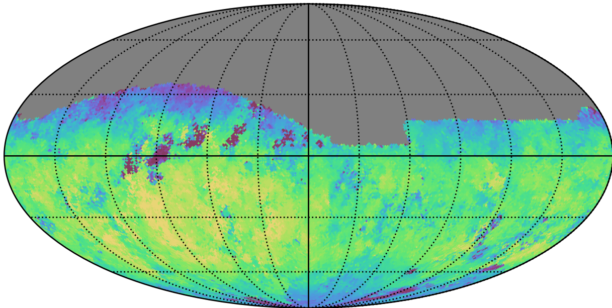
smc_lmc_v3.3_10yrs Yr 1 r band: Median fiveSigmaDepth
