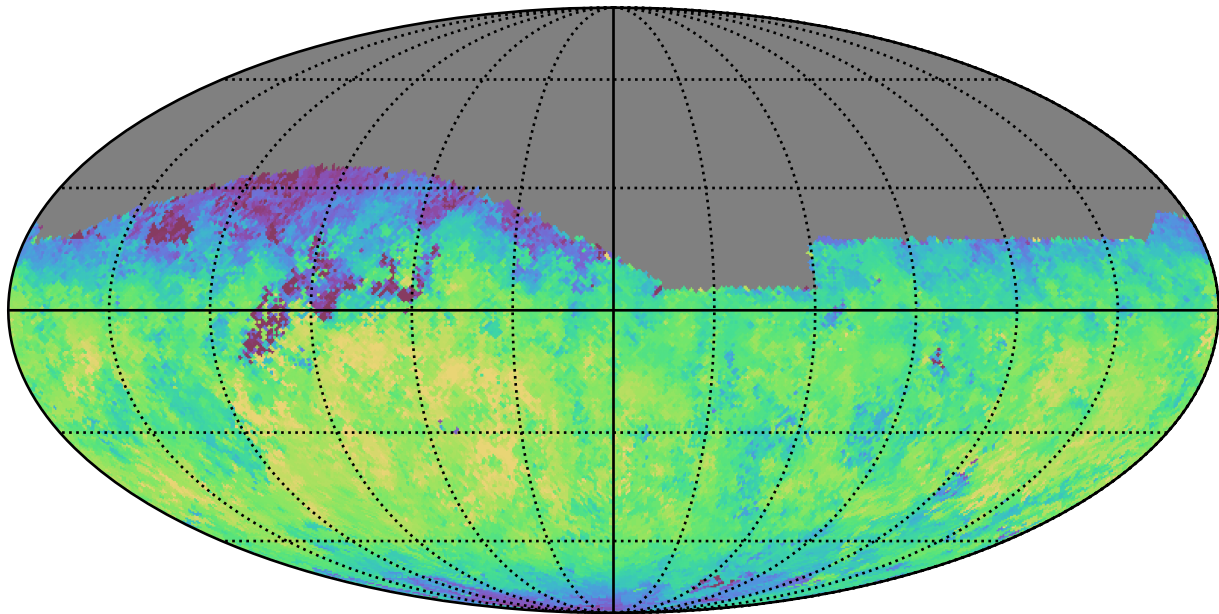
smc_lmc_v3.3_10yrs Yr 1 i band: Median fiveSigmaDepth
