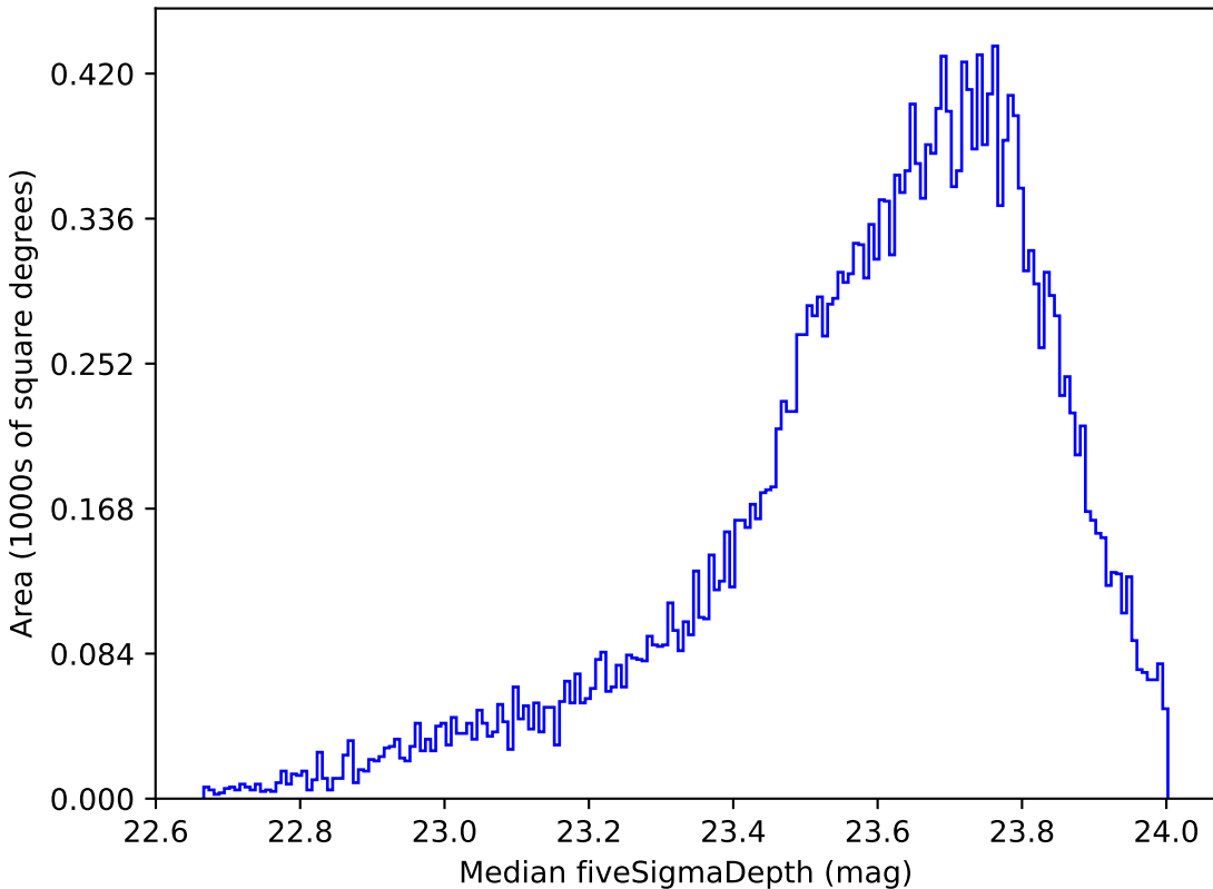
smc_lmc_v3.3_10yrs Yr 1 i band: Median fiveSigmaDepth
