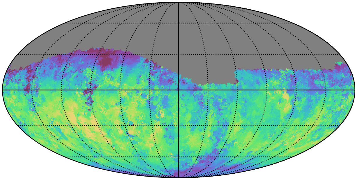
smc_lmc_v3.3_10yrs Yr 1 g band: Median fiveSigmaDepth
