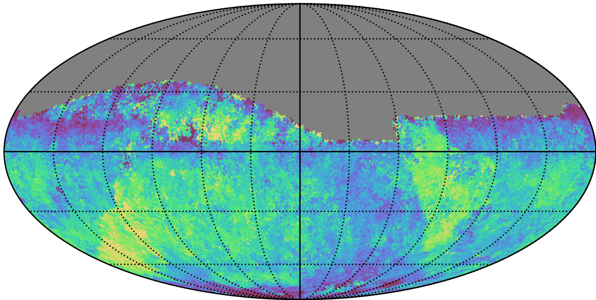
smc_lmc_v3.3_10yrs Yr 1 all bands: Median fiveSigmaDepth
