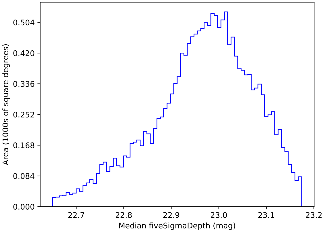
smc_lmc_v3.3_10yrs WFD z band: Median fiveSigmaDepth
