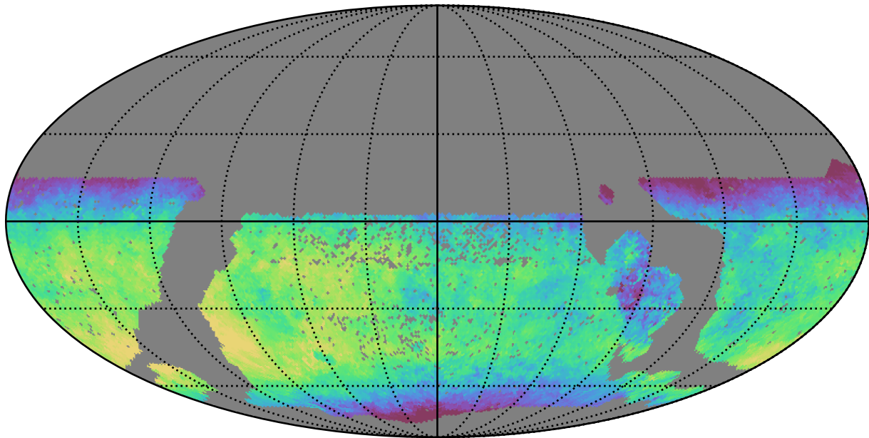
smc_lmc_v3.3_10yrs WFD y band: Median fiveSigmaDepth
