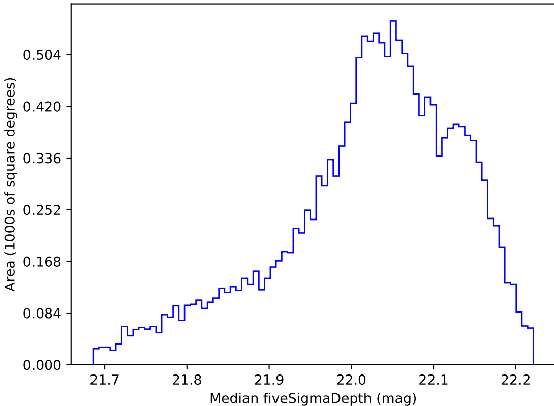
smc_lmc_v3.3_10yrs WFD y band: Median fiveSigmaDepth
