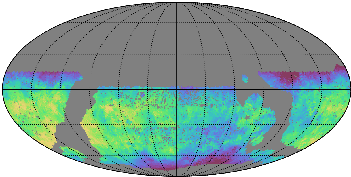
smc_lmc_v3.3_10yrs WFD u band: Median fiveSigmaDepth
