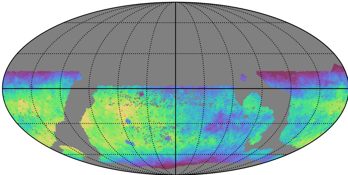
smc_lmc_v3.3_10yrs WFD r band: Median fiveSigmaDepth
