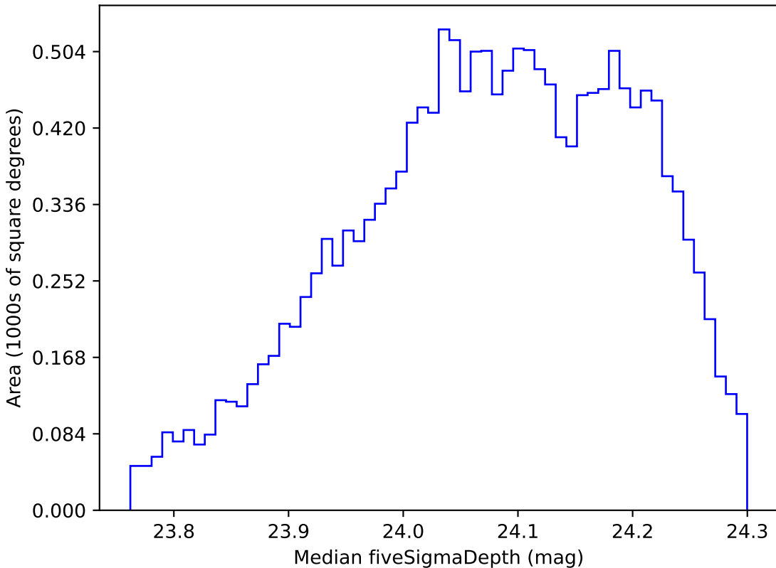
smc_lmc_v3.3_10yrs WFD r band: Median fiveSigmaDepth
