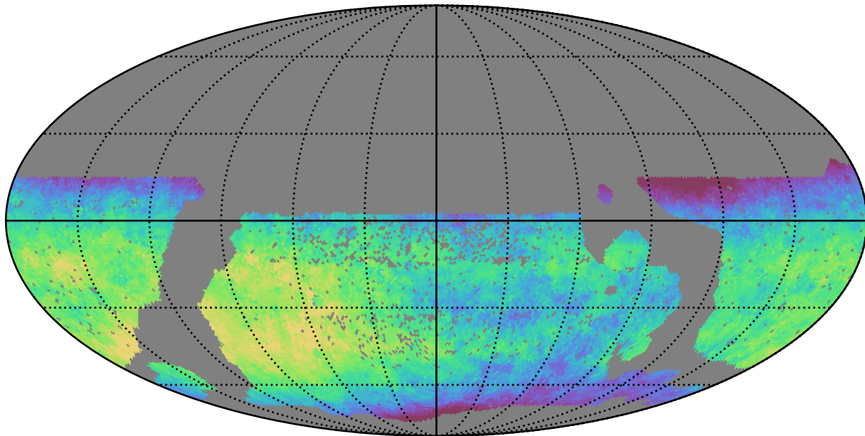
smc_lmc_v3.3_10yrs WFD i band: Median fiveSigmaDepth
