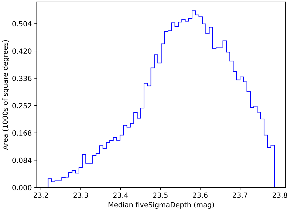
smc_lmc_v3.3_10yrs WFD i band: Median fiveSigmaDepth
