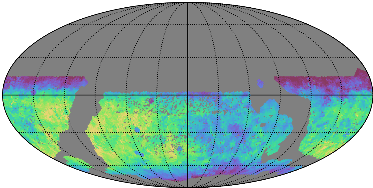
smc_lmc_v3.3_10yrs WFD g band: Median fiveSigmaDepth
