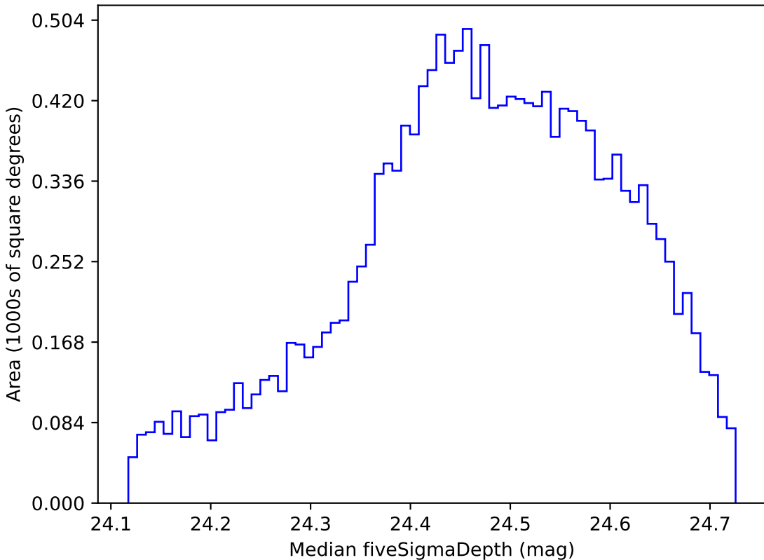
smc_lmc_v3.3_10yrs WFD g band: Median fiveSigmaDepth
