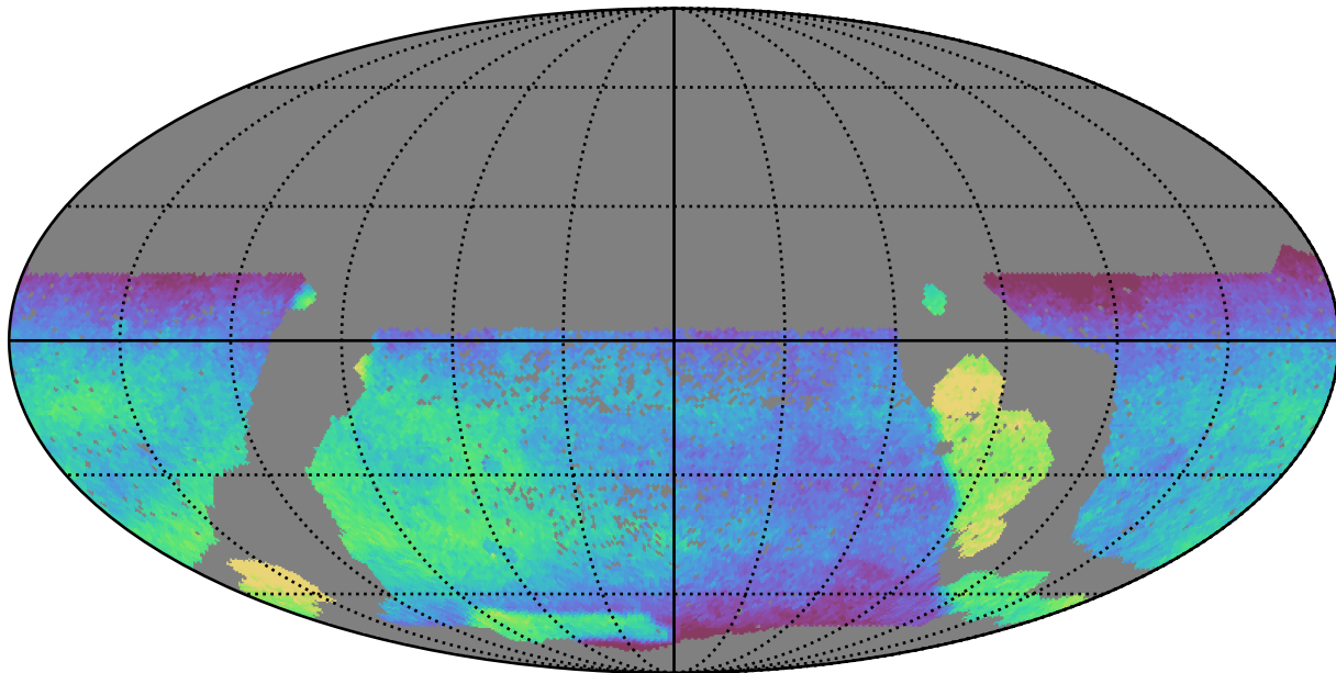
smc_lmc_v3.3_10yrs WFD all bands: Median fiveSigmaDepth
