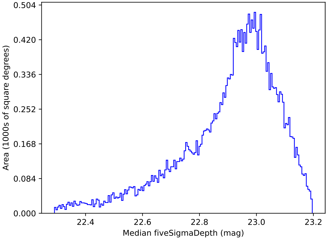
smc_lmc_v3.3_10yrs All sky z band: Median fiveSigmaDepth
