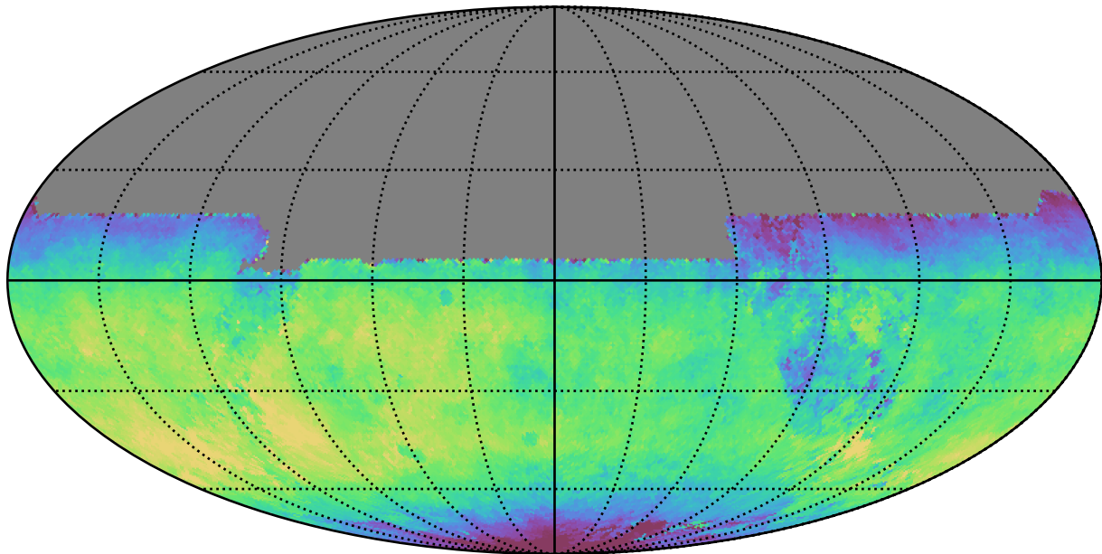
smc_lmc_v3.3_10yrs All sky y band: Median fiveSigmaDepth
