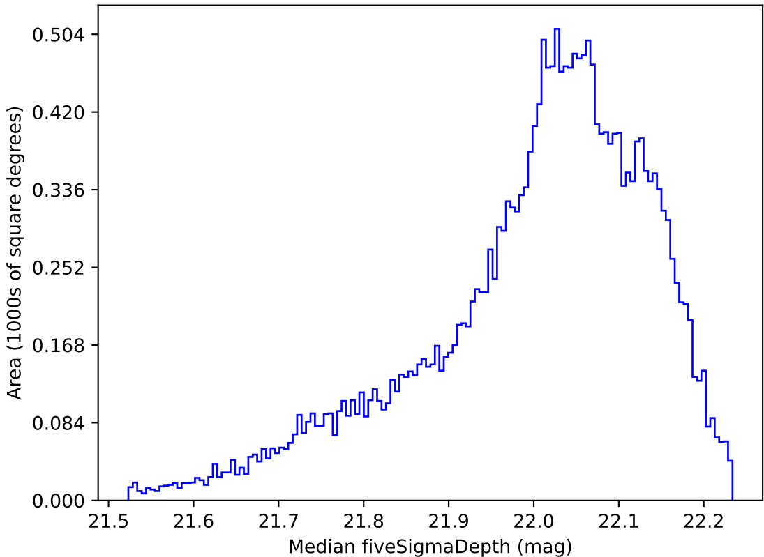
smc_lmc_v3.3_10yrs All sky y band: Median fiveSigmaDepth
