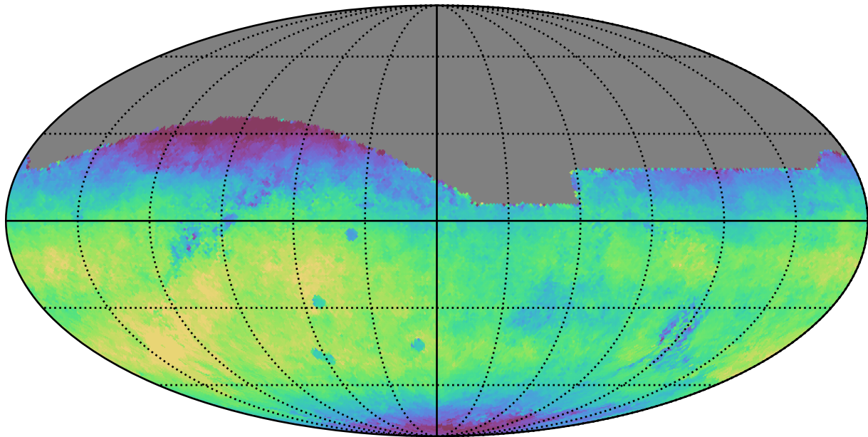
smc_lmc_v3.3_10yrs All sky r band: Median fiveSigmaDepth
