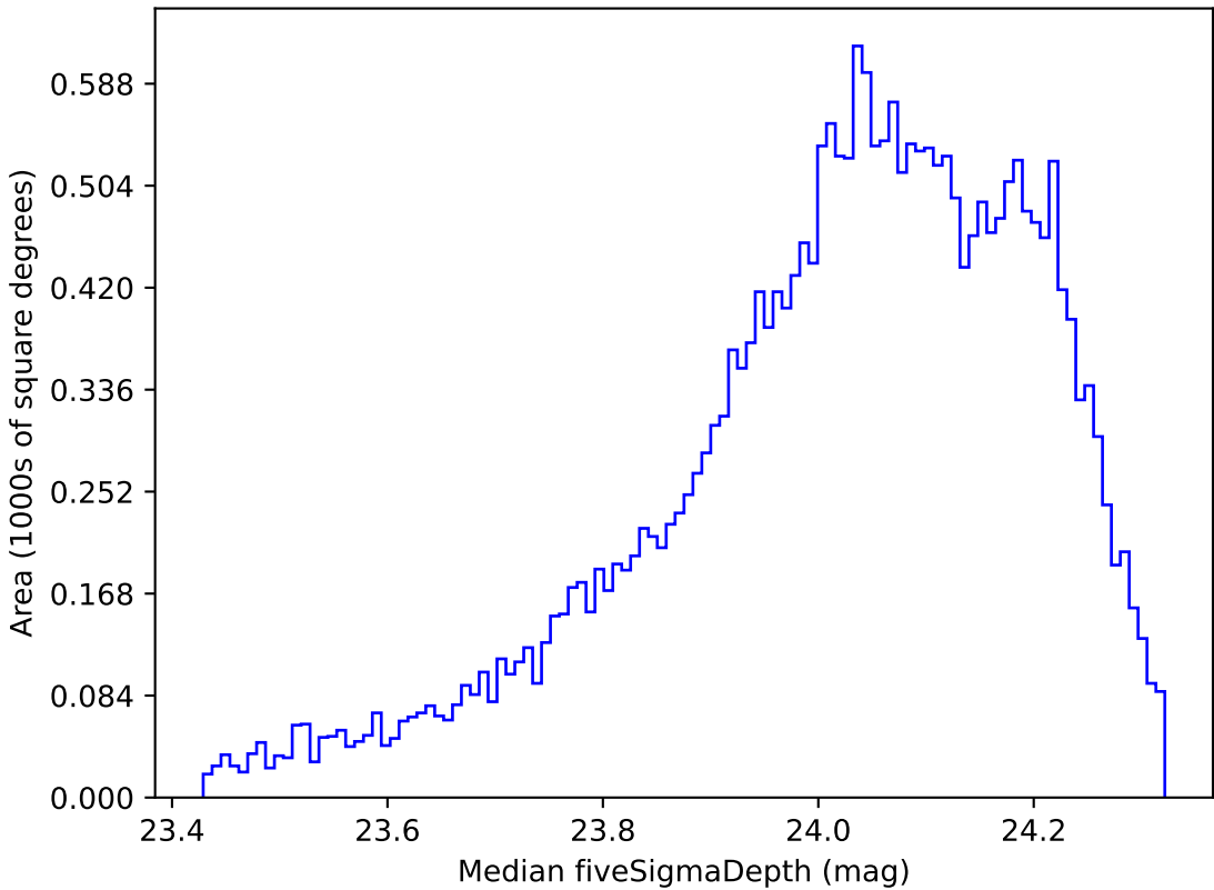
smc_lmc_v3.3_10yrs All sky r band: Median fiveSigmaDepth
