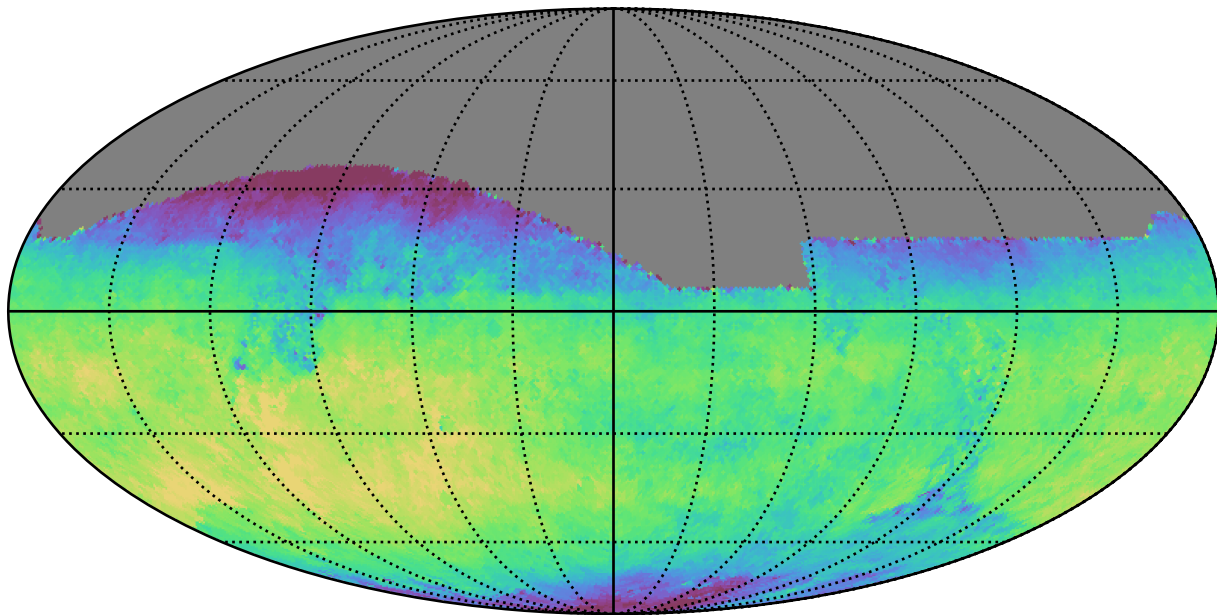
smc_lmc_v3.3_10yrs All sky i band: Median fiveSigmaDepth
