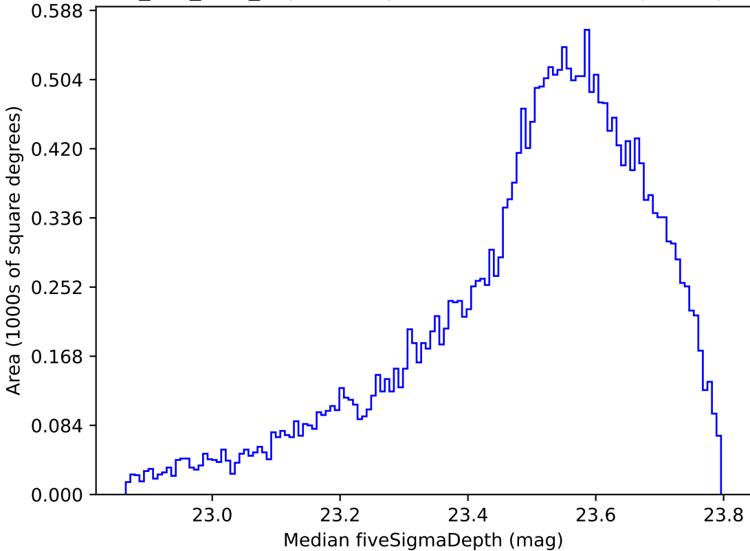
smc_lmc_v3.3_10yrs All sky i band: Median fiveSigmaDepth
