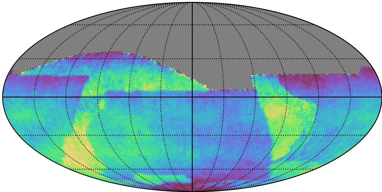
smc_lmc_v3.3_10yrs All sky all bands: Median fiveSigmaDepth
